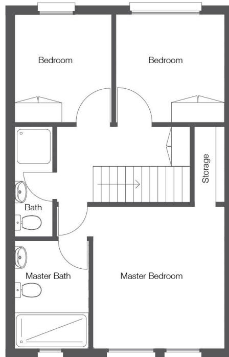
SECOND FLOOR
